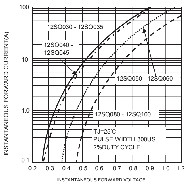
FIG.4-TYPICAL FORWARD CHARACTERISTICS
